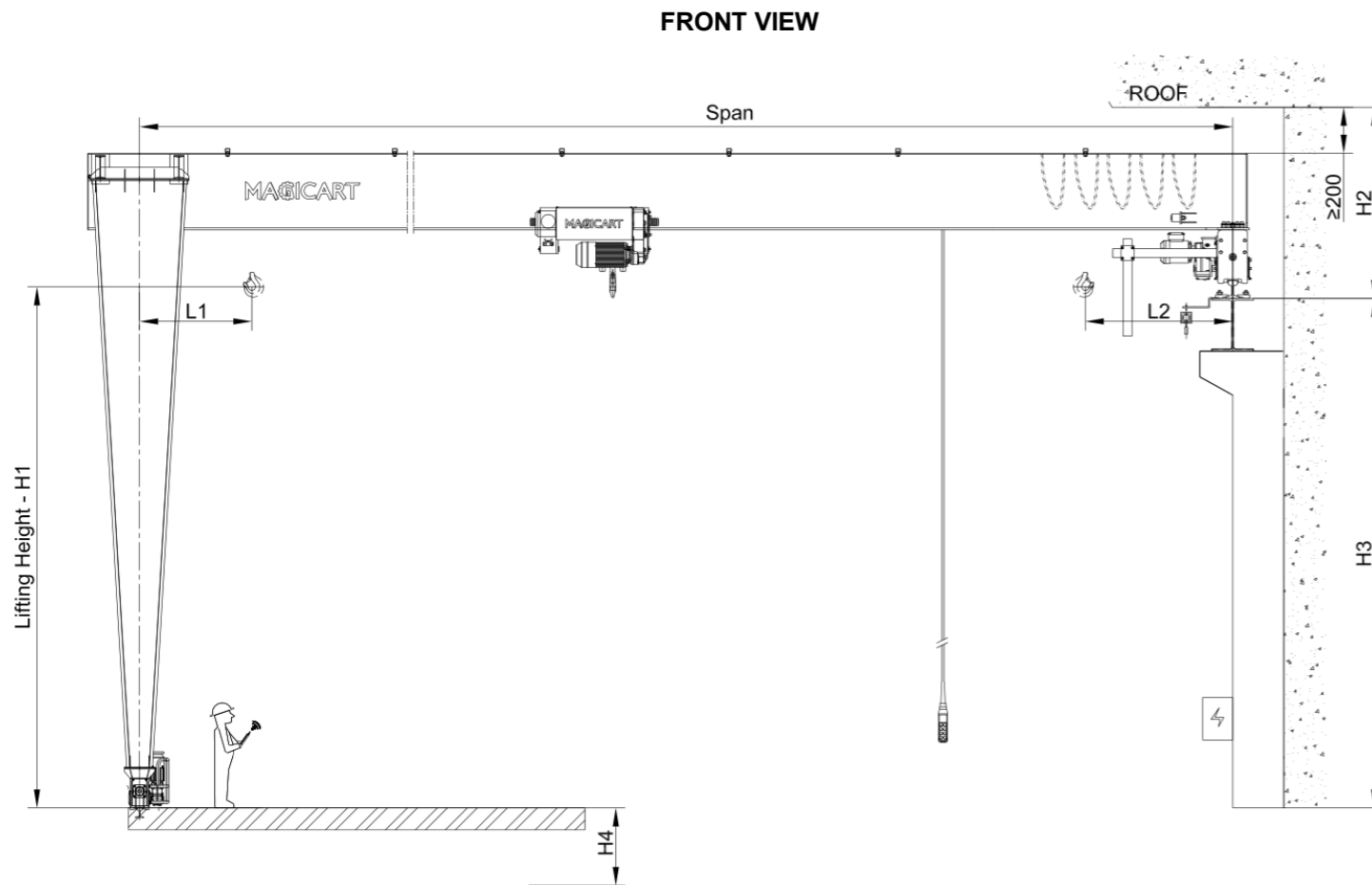
CRANE LAYOUT
