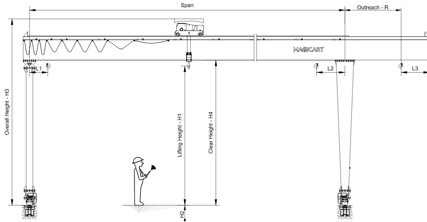
CRANE LAYOUT
