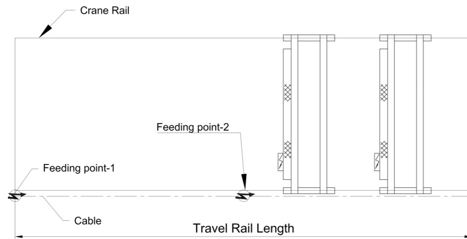
CRANE LAYOUT
